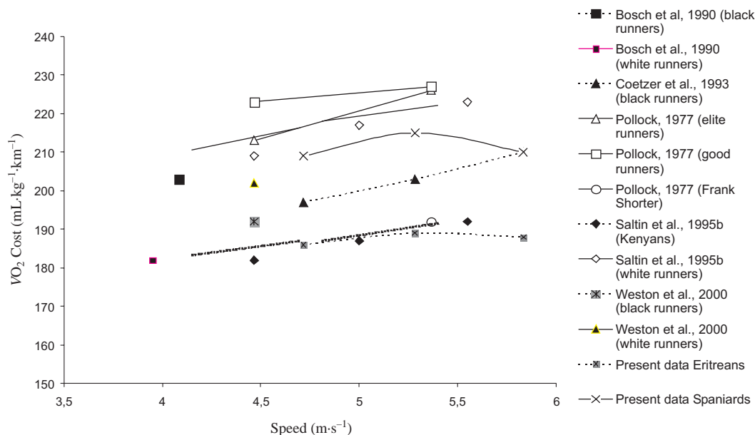
Fig. 1. Comparison of the profile of the running VO_2 cost (in our subjects (Eritreans and Spaniards)) and in those of previous research on elite runners. For studies conducted during level treadmill running, the VO_2 cost ( mL\ O_2 \cdot kg^{-1} \cdot km^{-1} ) was adjusted to 1% grade based on the model used by the ACSM (American College of Sports Medicine 2000), where VO_2 ( mL \cdot kg^{-1} \cdot m^{-1} ) at 1% for a given speed = VO_2 ( mL \cdot kg^{-1} \cdot m^{-1} ) at 0% for the same speed ( m \cdot min^{-1} ) + ( m \cdot min^{-1} \times 0.9 \times 0.01 ).
